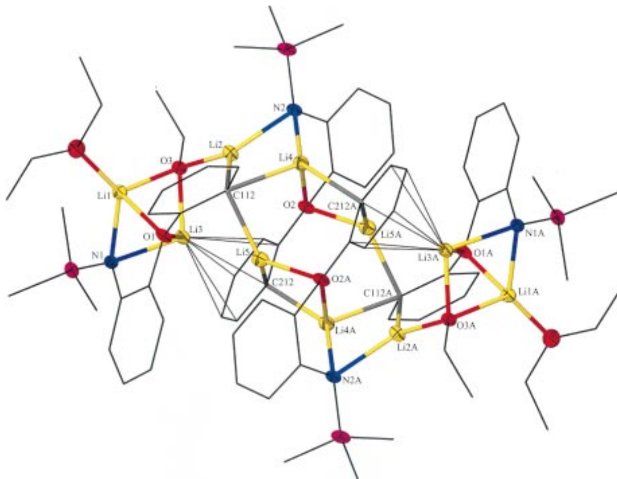
Figure 1. Molecular structure of \mathbf{1} \cdot \text{hexane} with the thermal ellipsoids shown at 30% probability level for the non-carbon atoms. For clarity, the molecule of hexane and the hydrogen atoms have been omitted and the carbon atoms are represented by lines.
